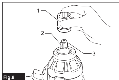
Fig. 8 ► 1. Impact socket 2. Square drive 3. Ring spring
