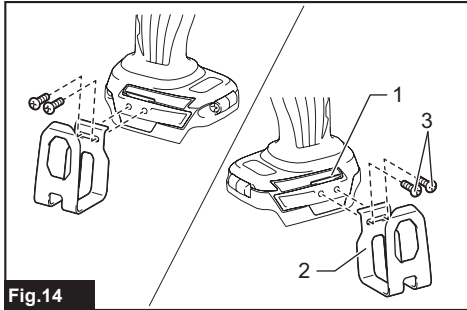
Fig.14 ► 1. Groove 2. Hook 3. Screw
