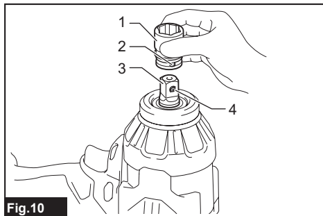
Fig. 10 ► 1. Impact socket 2. Hole 3. Square drive 4. Detent pin
