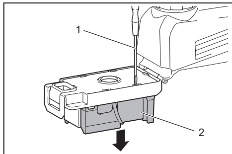
► 1. Flat-blade screwdriver 2. Filter case
