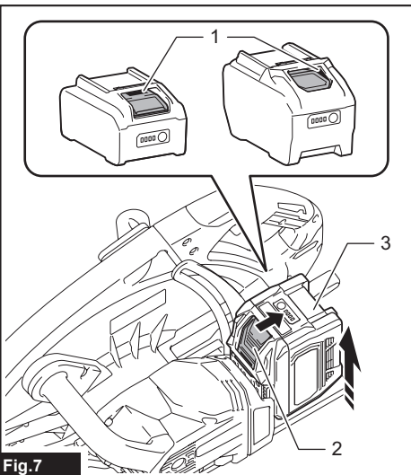
Fig.7 ► 1. Red indicator 2. Button 3. Battery cartridge
